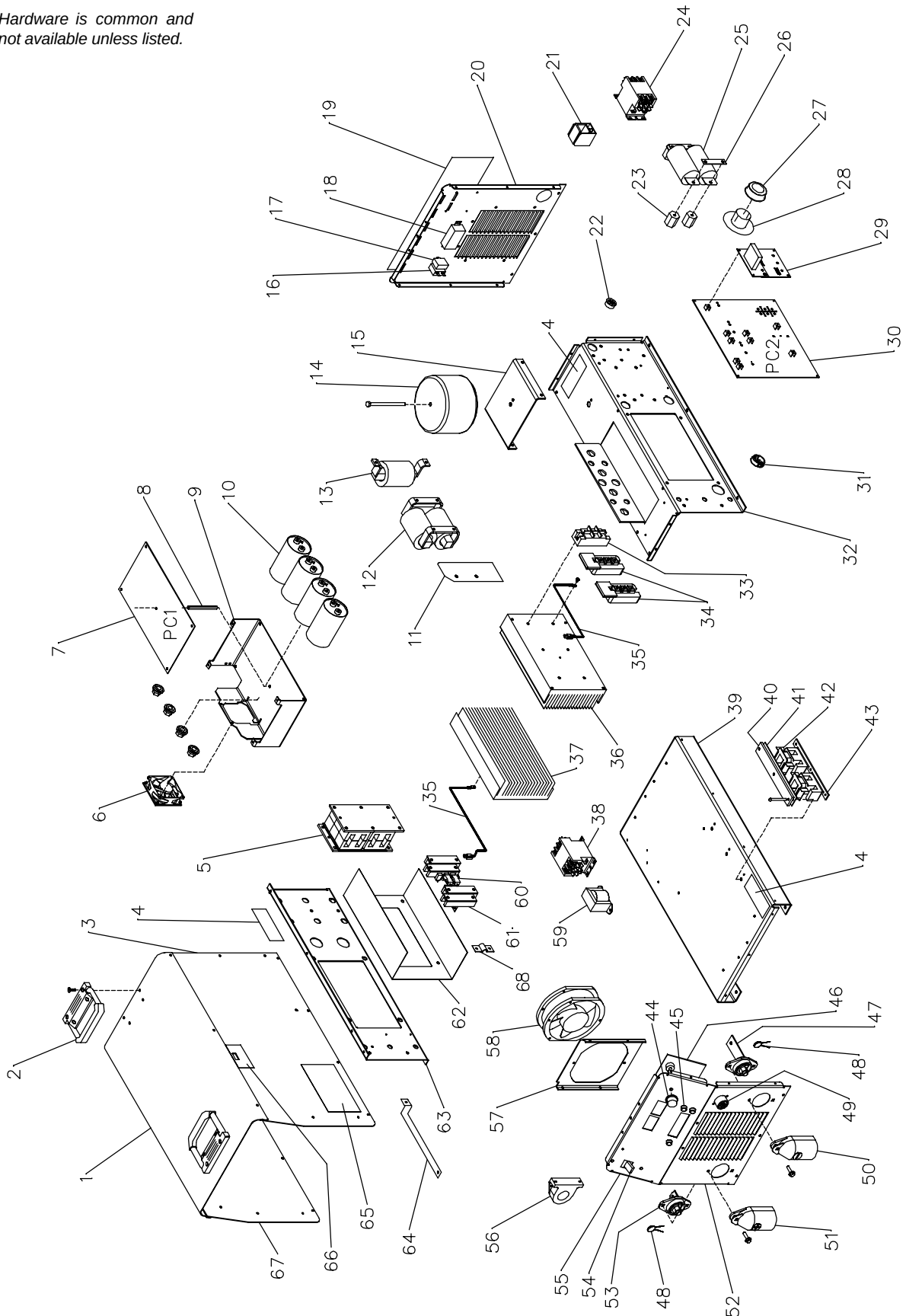
Figure 7-1. Complete Assembly
